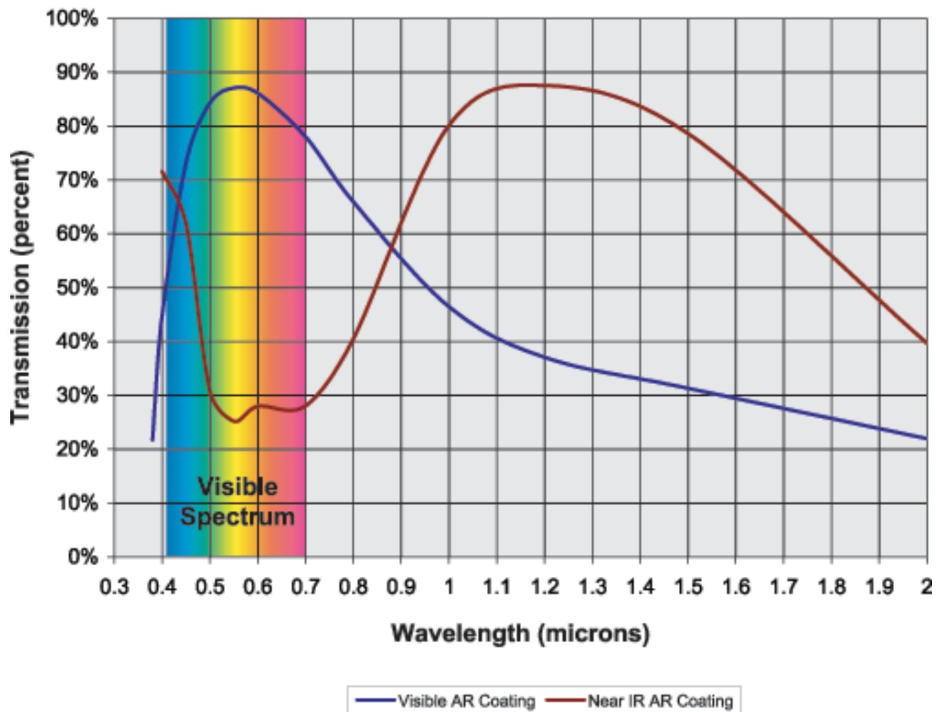
Transmission of the 12x zoom lens
