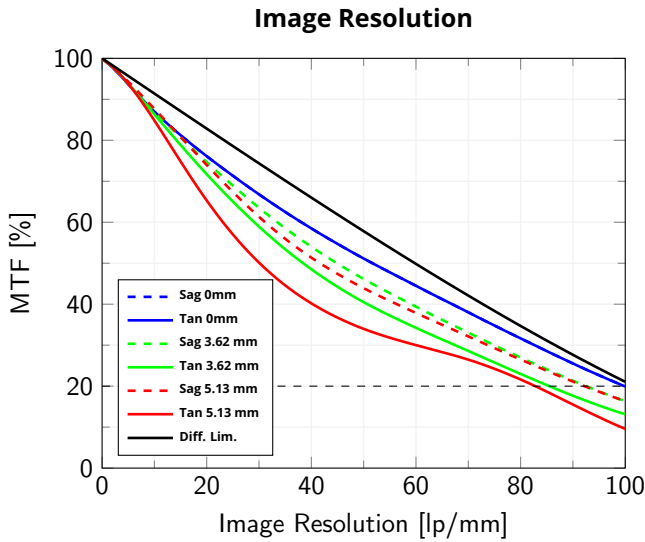
Modulation Transfer Function (MTF) vs. Image Resolution, wavelength range 400-700 nm, wf/N = 11.5
