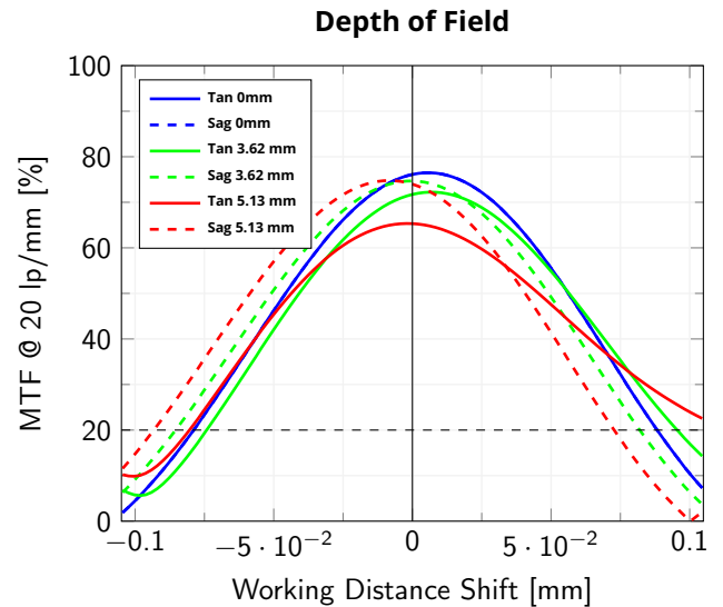
Modulation Transfer Function (MTF) @ 20 lp/mm vs. Working Distance Shift from the best focus Working Distance, wavelength range 400-700 nm, wf/N = 11.5
