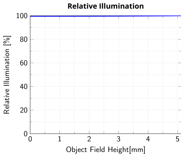
Relative illumination vs. Object Field Height, from the optical axis to the corner of the field of view, wf/N = 11.5
