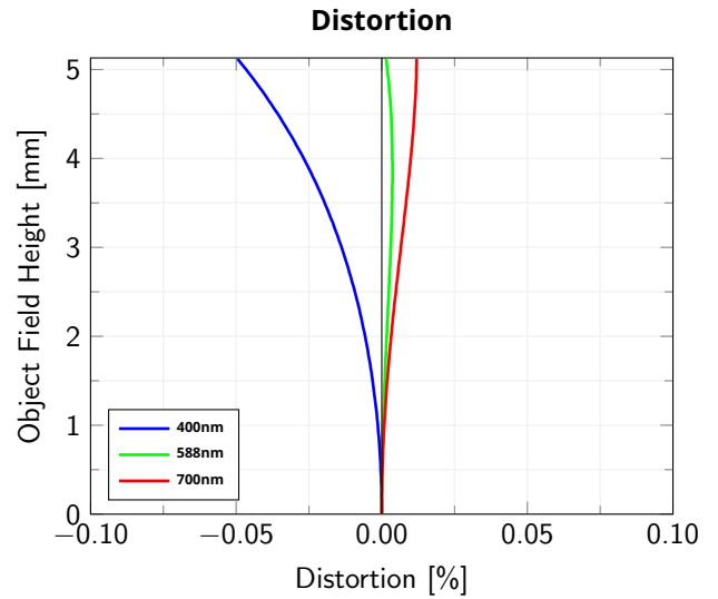
Object Field Height vs. Distortion, from the optical axis to the corner of the field of view, wf/N = 11.5
