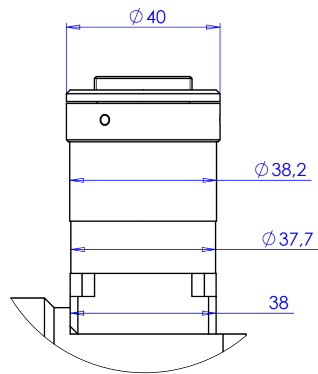
DETAIL C SCALE 1:1
