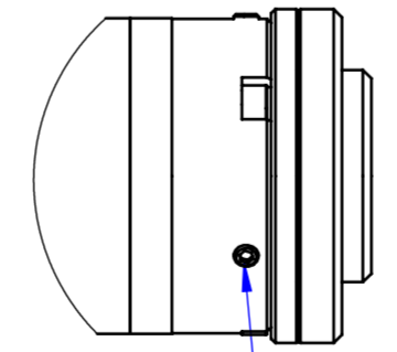
DETAIL D SCALE 1 : 1 Phase adjustment
