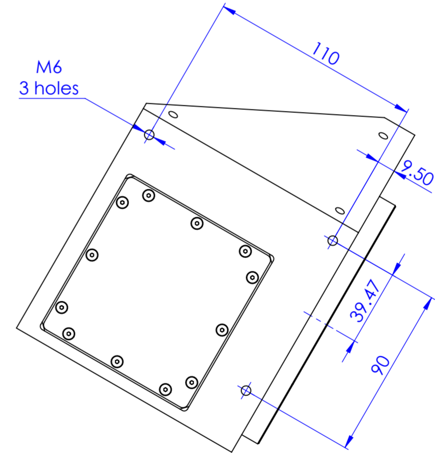
VIEW A
