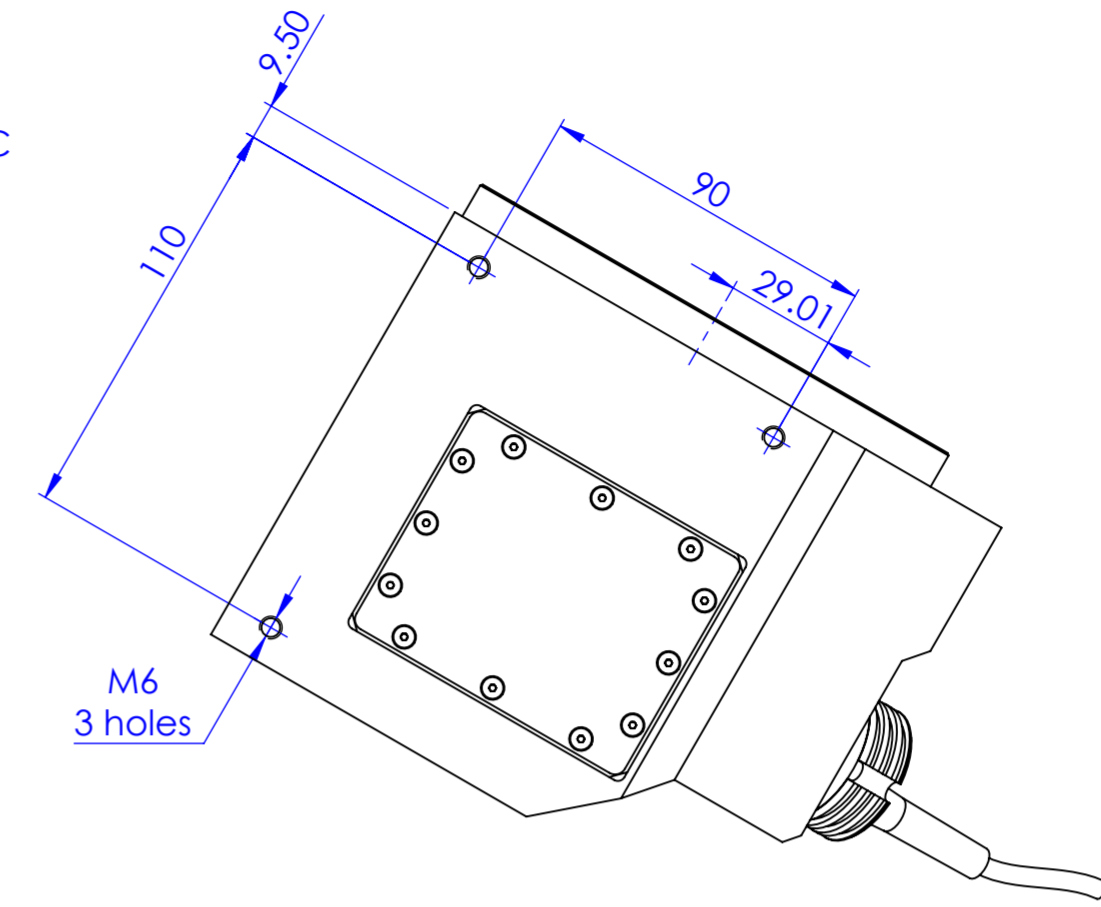
VIEW C
