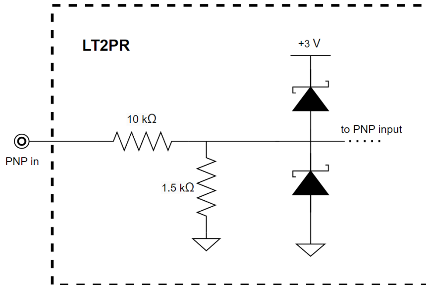
Figure 21: Scheme of the PNP input.
