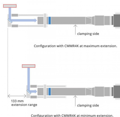
CMMR4K-V bends the light rays vertically. UPWARD BEND
