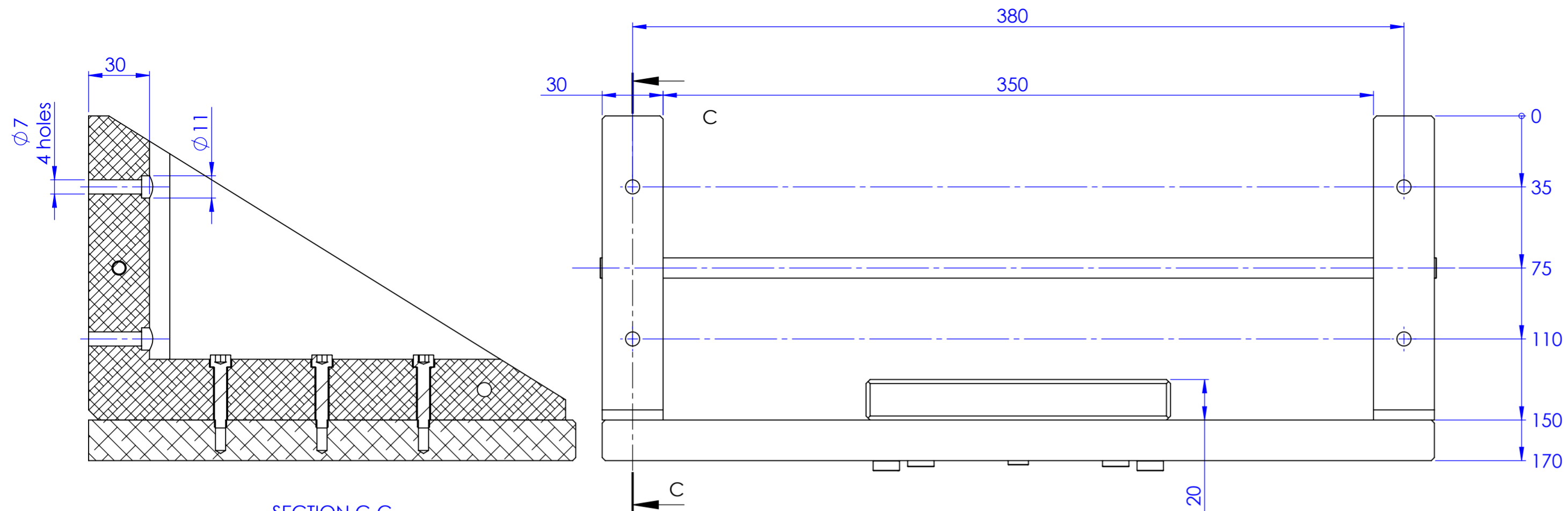
SECTION C-C
