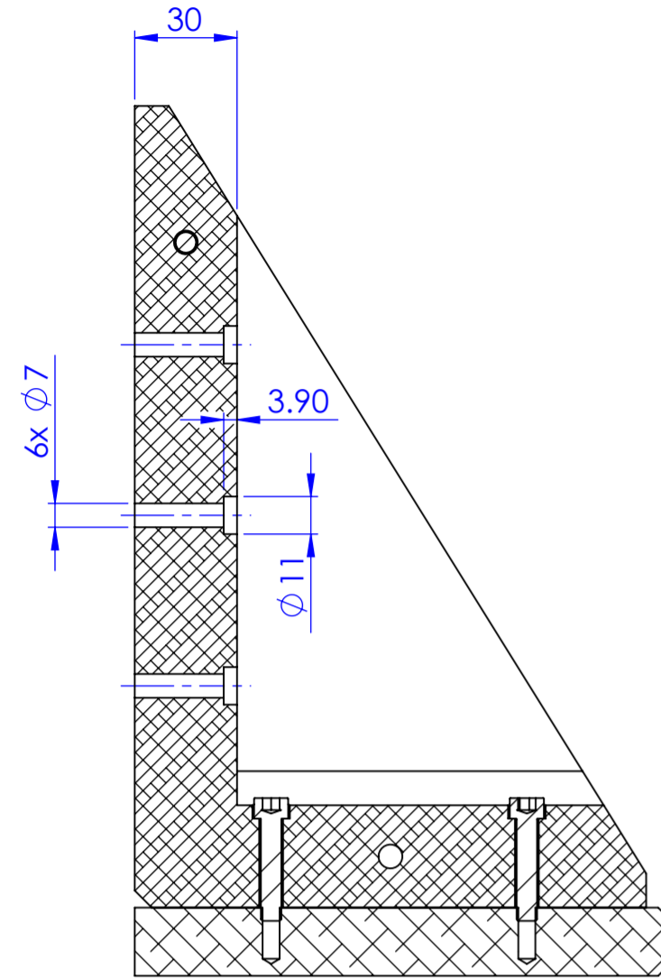
SECTION C-C
