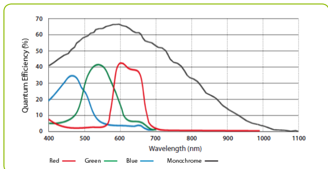
Color response includes IR-cut filter
