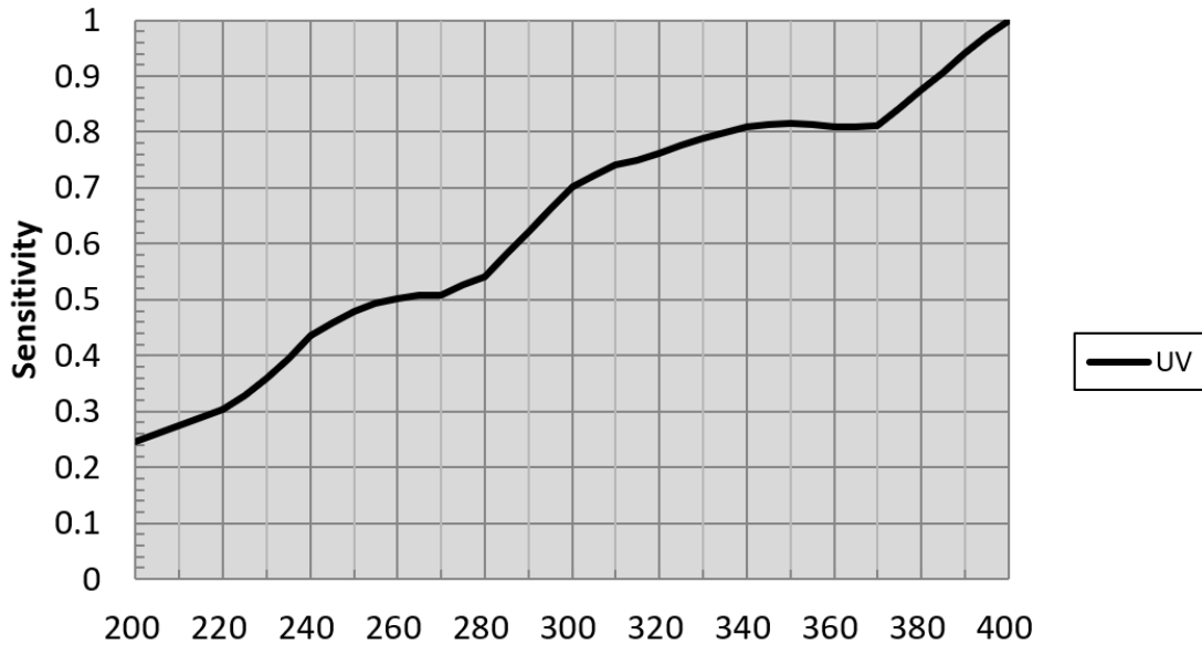
GO-8105M-UV Sensitivity
