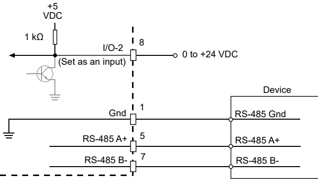
I/O Schematic, Variant 2 (Input Port Connected to Input Voltage)
