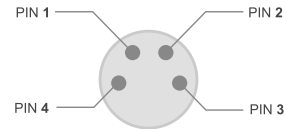
Device side - male pins Front view
